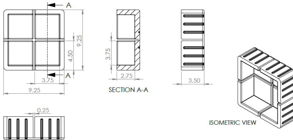
0.75-inch Standard Corner Set Drawings
