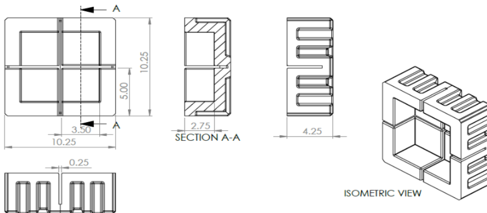
1.5-inch Standard Corner Set Drawings
